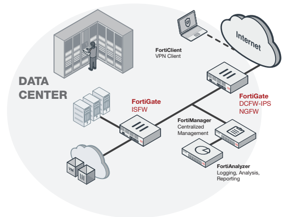
FortiGate 3960E/3980E deployment in data center (DCFWS-IPS/NGFW, ISFW)
